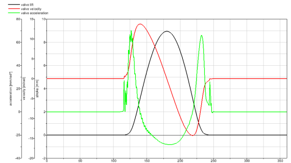
single valvetrain results
